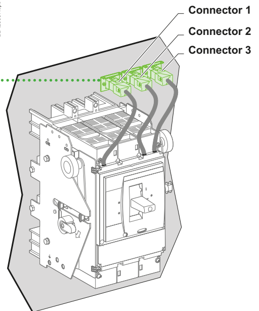
ComPact NSX400/630.
