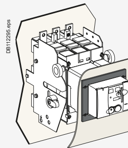
Standard escutcheon for motor mechanism.
